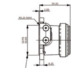
PISTON FULLY RETRACTED
