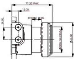
PISTON AT MAXIMUM STROKE
