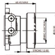
PISTON AT FULL STROKE
