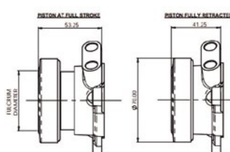
REDUCED LENGTH CONFIGURATION (12mm STROKE)
