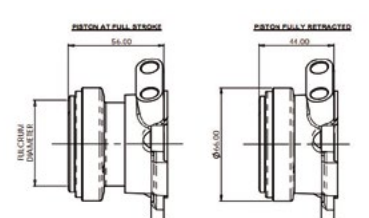
REDUCED LENGTH - INNER ROTATING RACE (12 mm STROKE)
