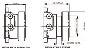
REDUCED LENGTH CONFIGURATION (12mm STROKE)
