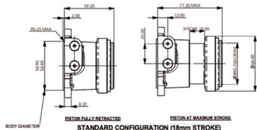
STANDARD CONFIGURATION (18mm STROKE)
